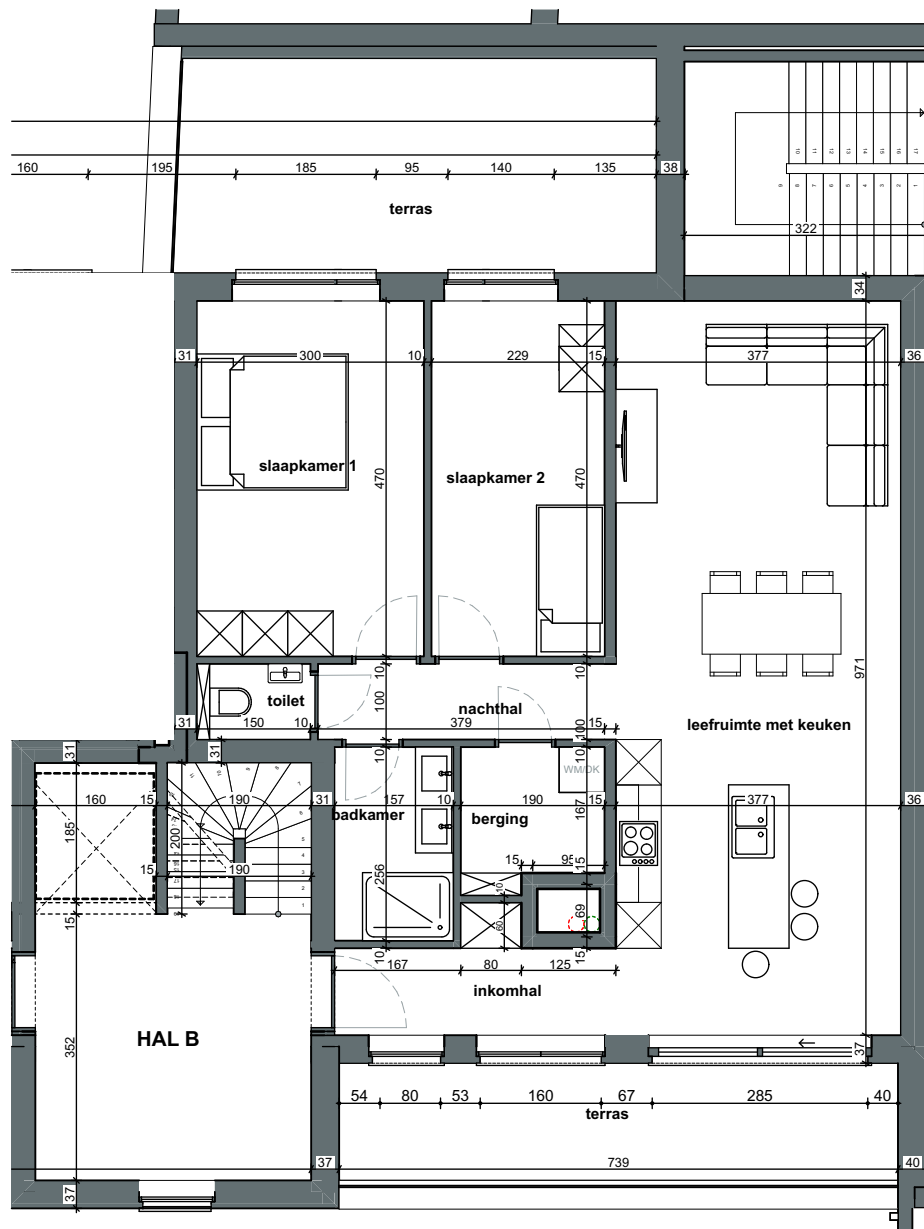
Verdieping 1 - B-B1.2 1:100
