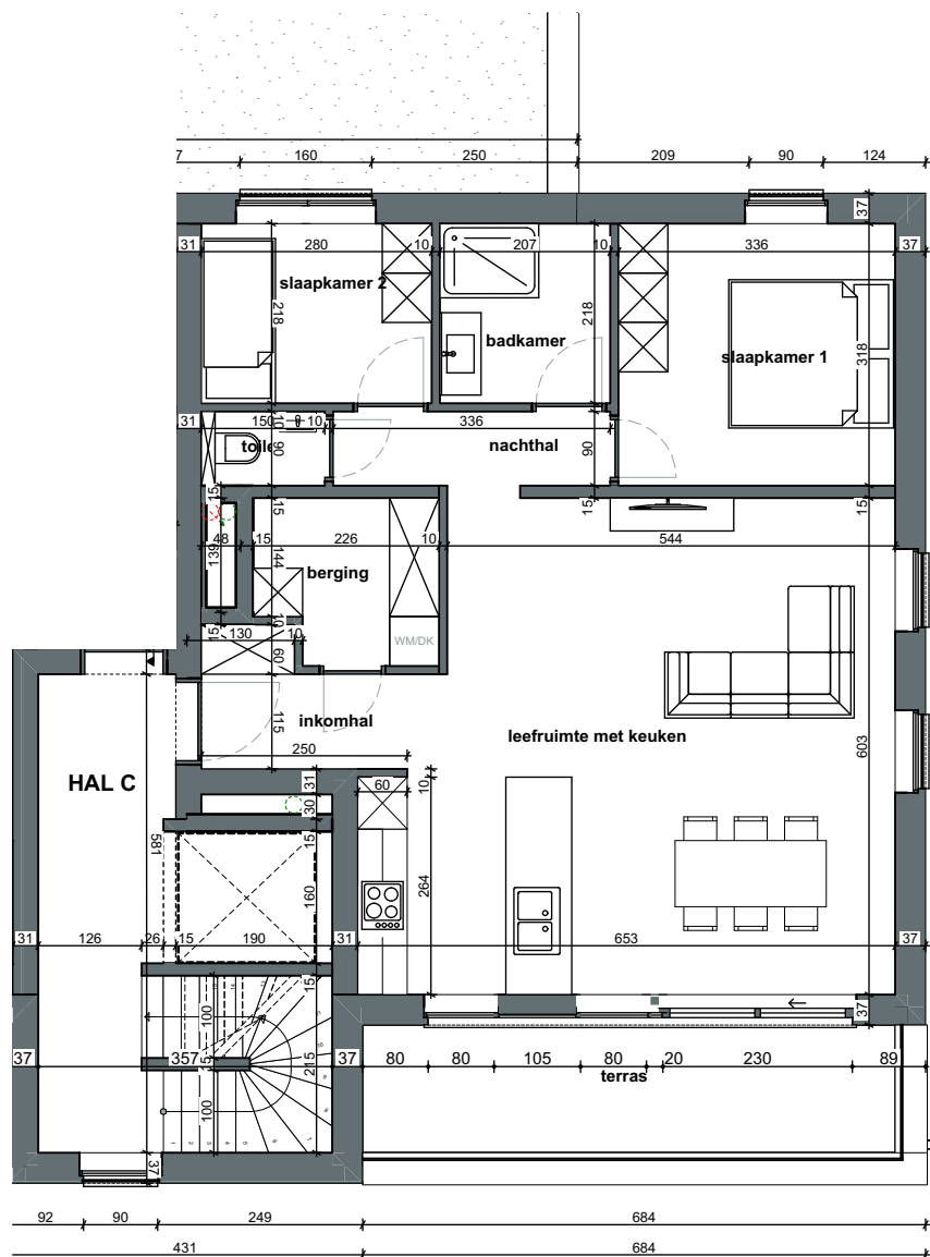
Verdieping 1 - B-C1.2 1:100
