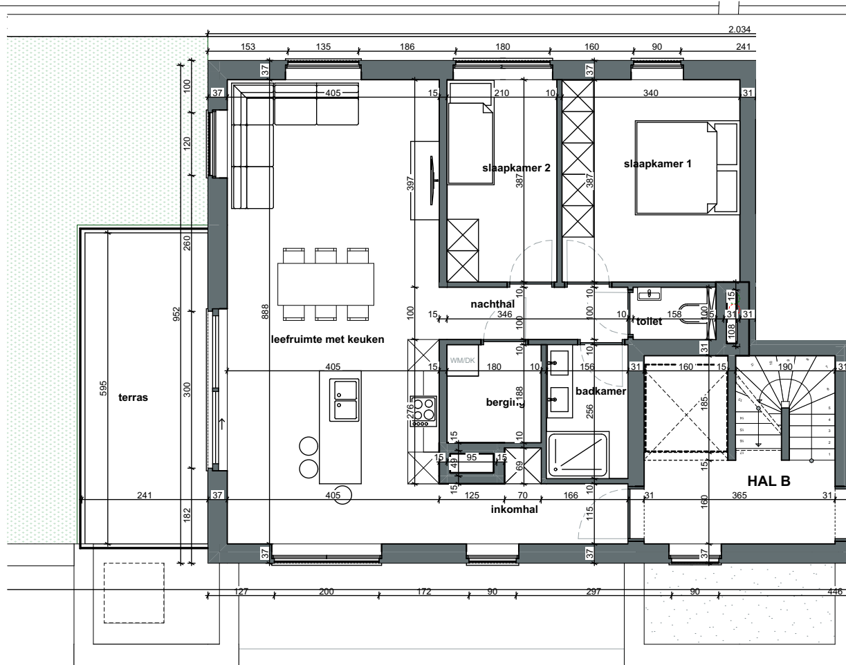
Verdieping 2 - B-B2.1 1:100
