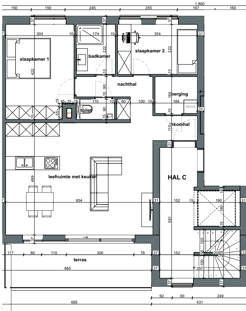
Verdieping 2 - B-C2.1 1:100
