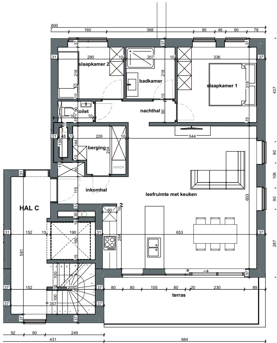
Verdieping 2 - B-C2.2 1:100
