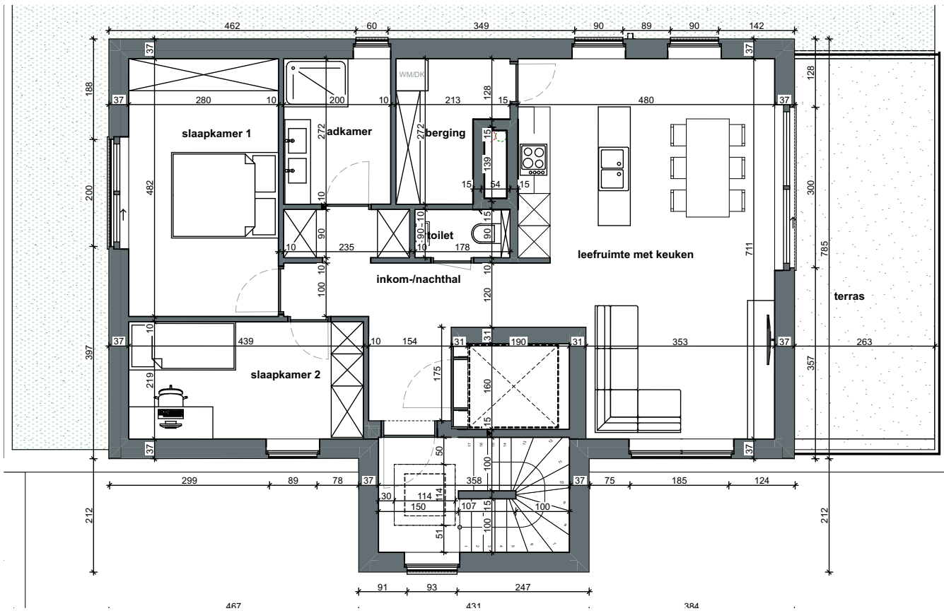
Verdieping 3 - B-C3.1 1:100
