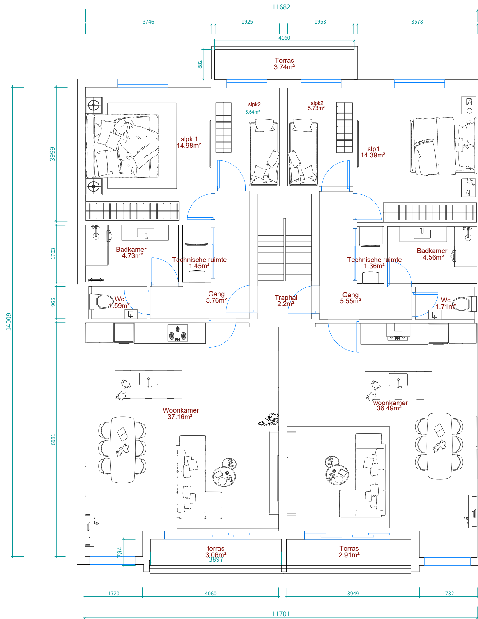
Furniture Plan(1:70)
