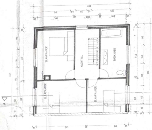
VERDEPING
