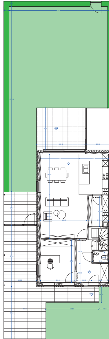
Inplanting
