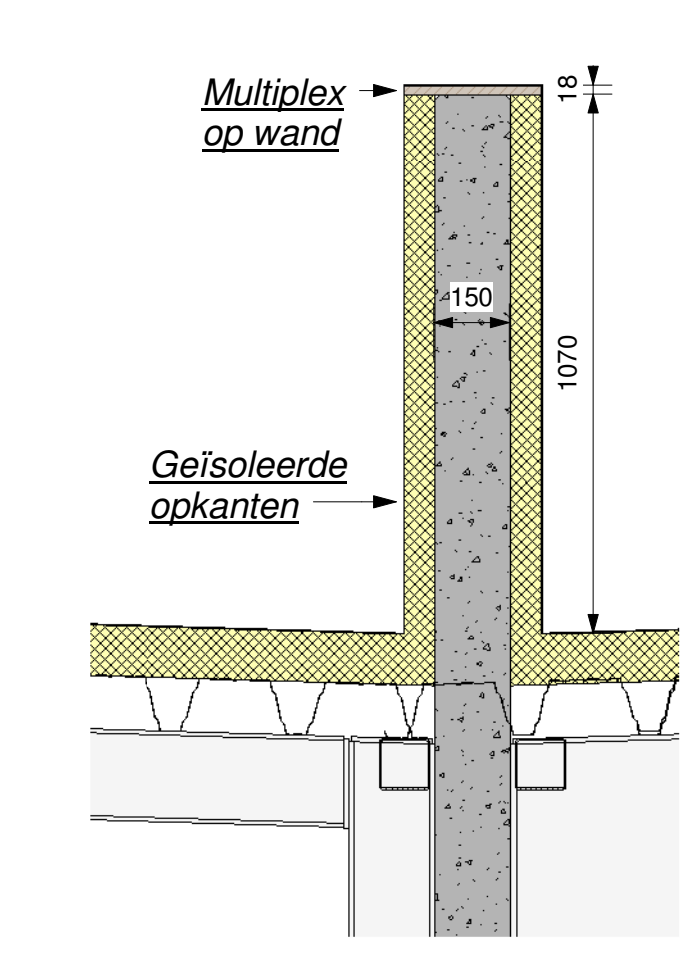
A Detail brandwand 1 : 15
