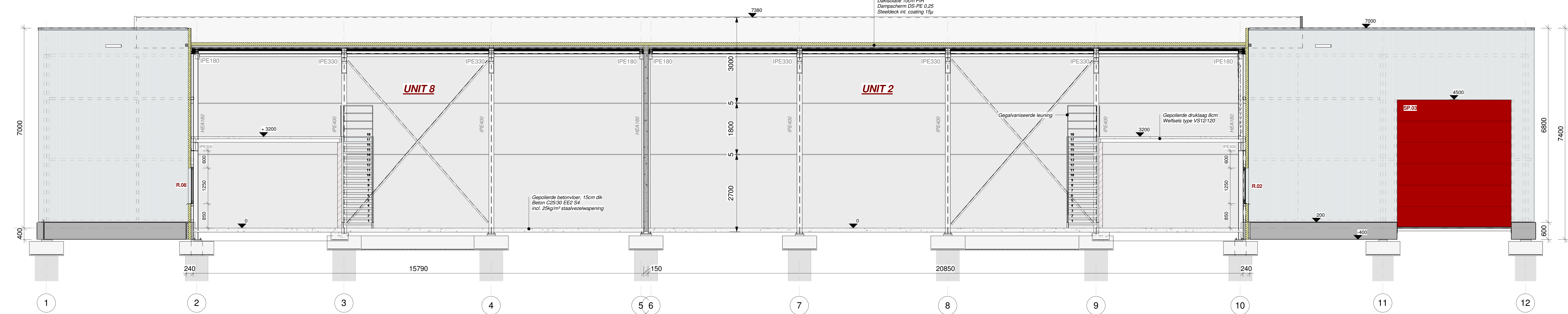
3 Snede as K 1 : 50
