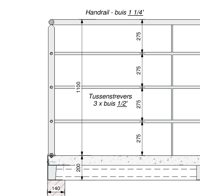
C Stortrand + leuning 1 : 15
