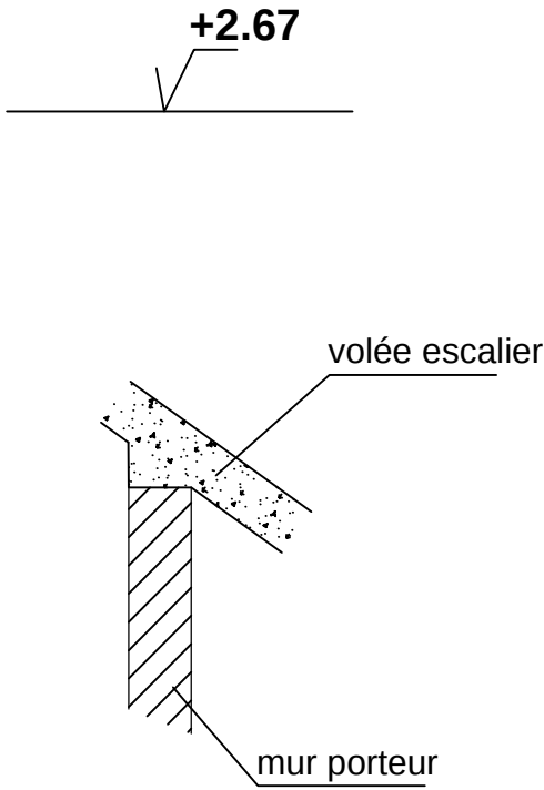
COUPE 2'-2'
