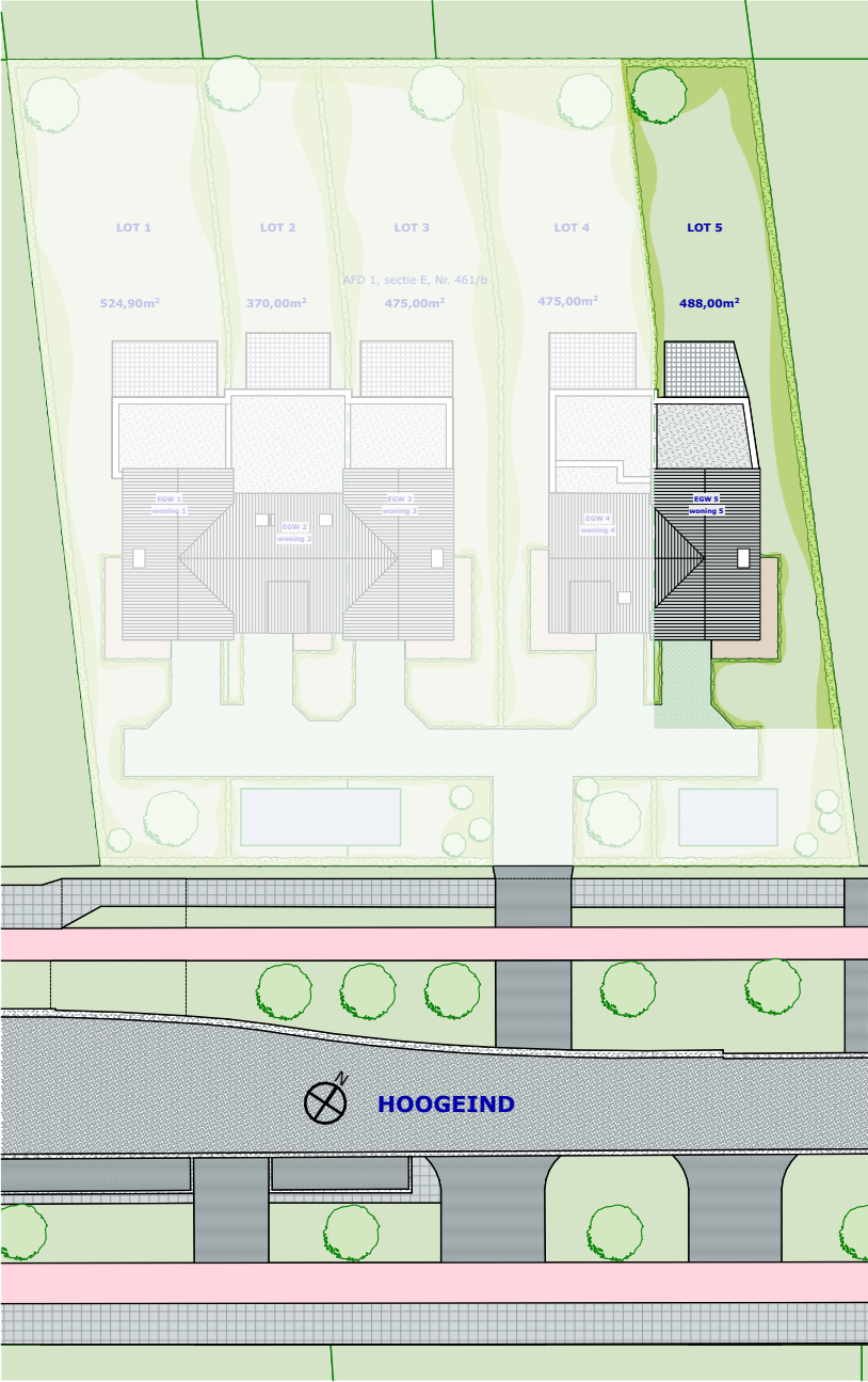
Inplantingsplan - 1:500
