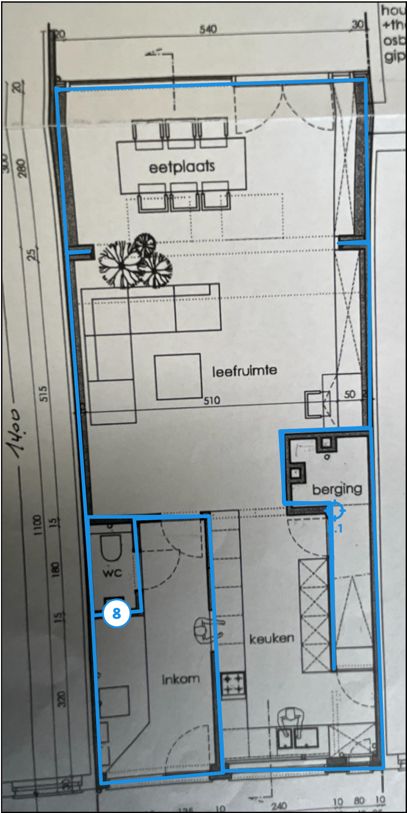
Legende van plan 1.1: Plan woning gvl
