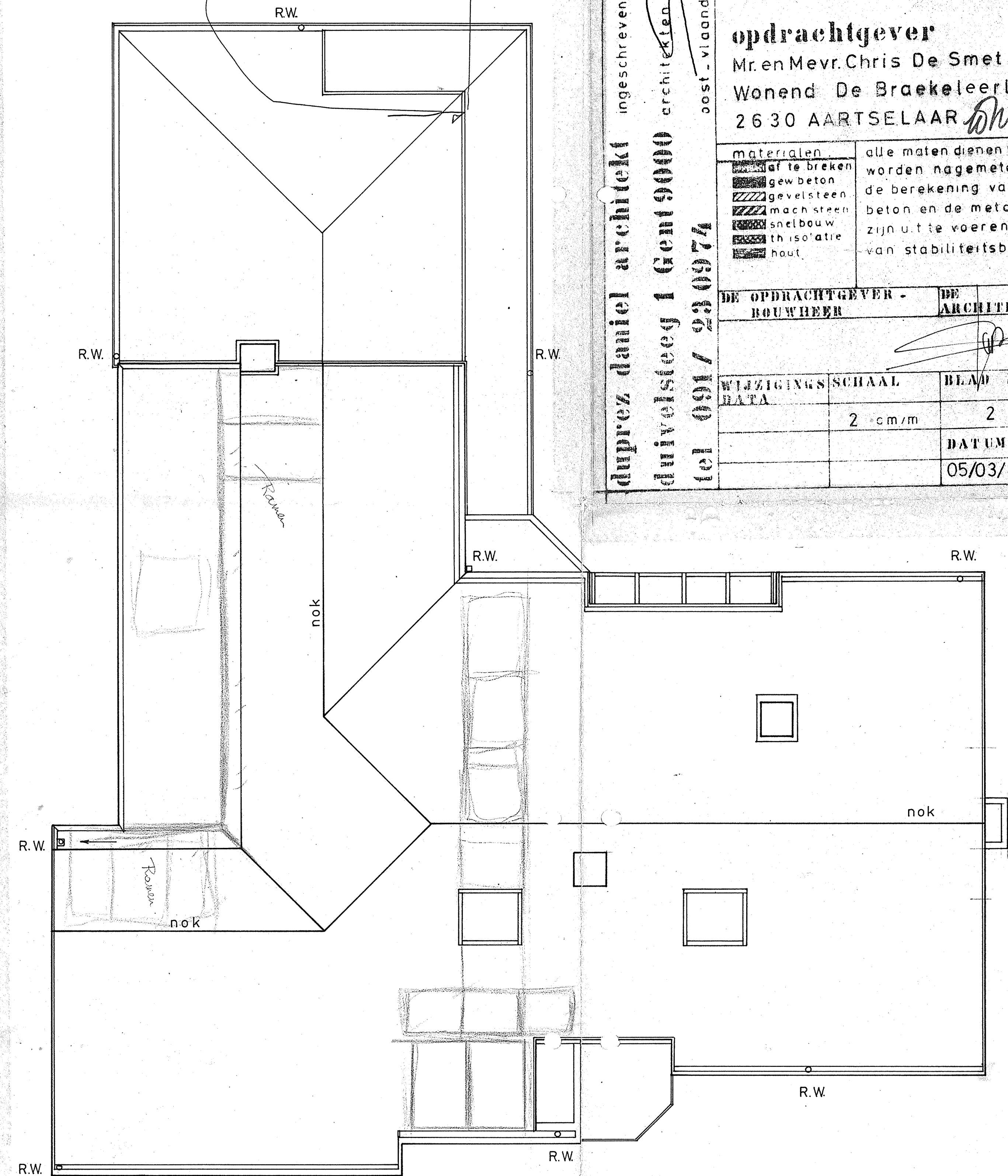
DAKENPLAN
