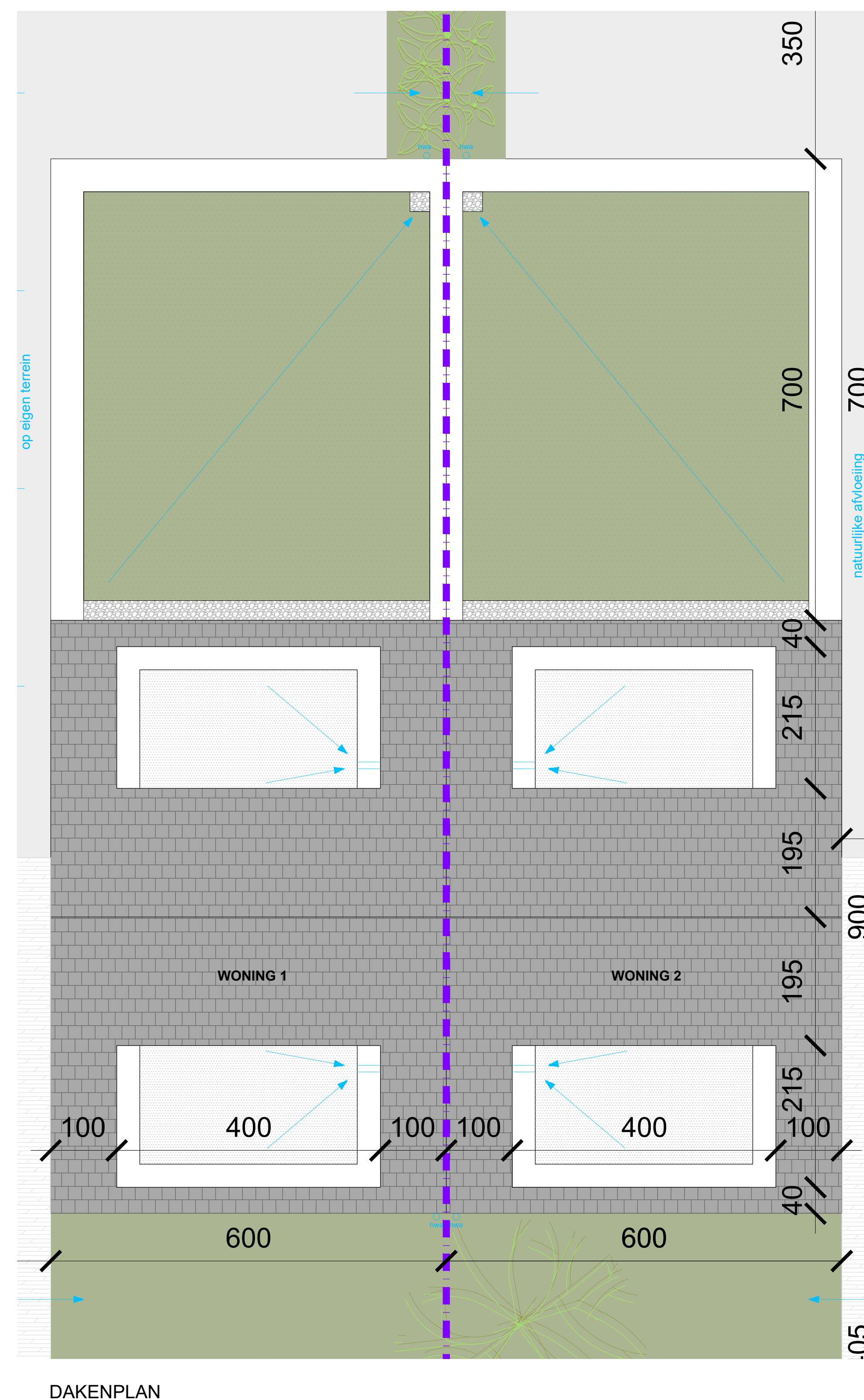
DAKENPLAN
