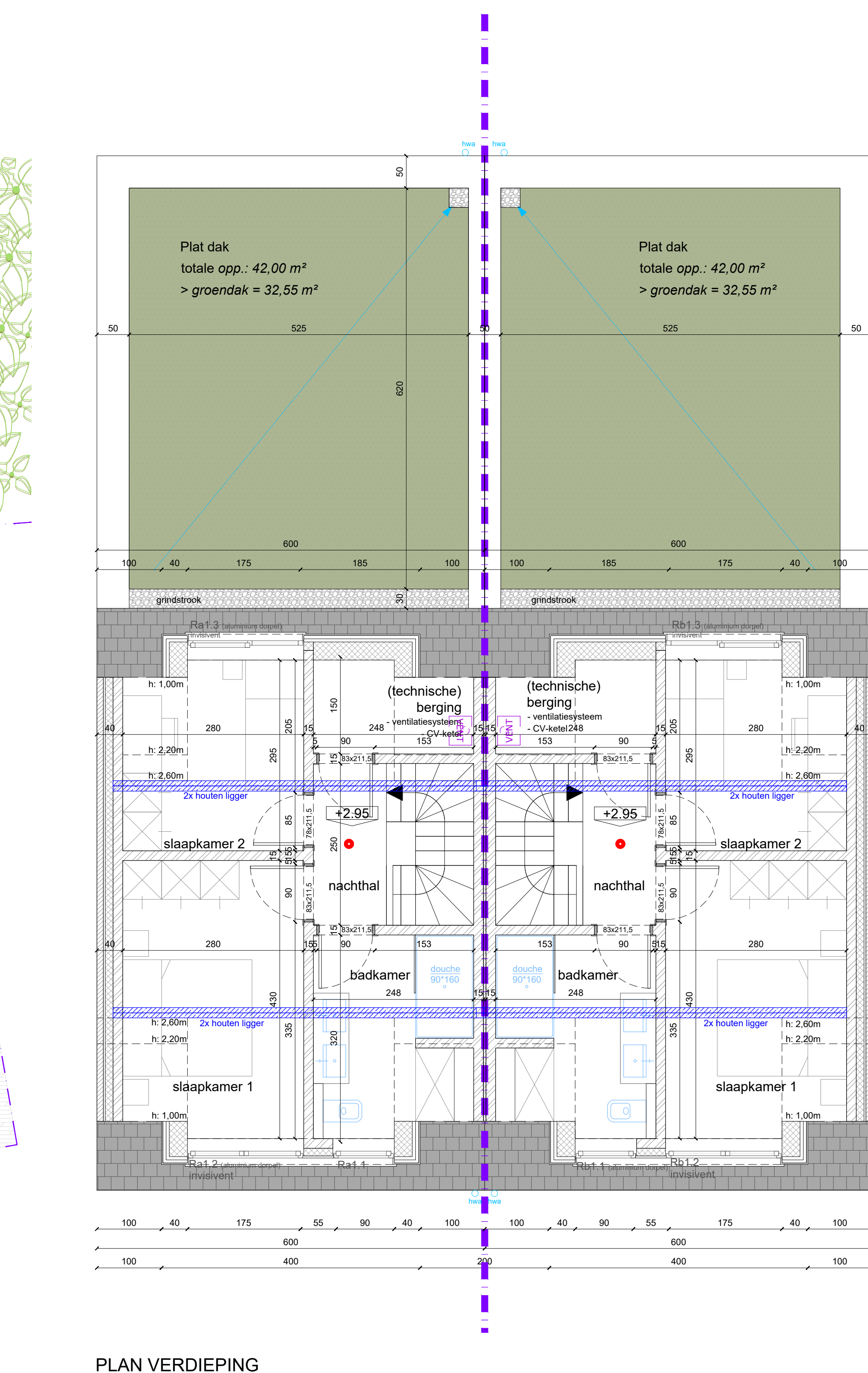
PLAN VERDIEPING
