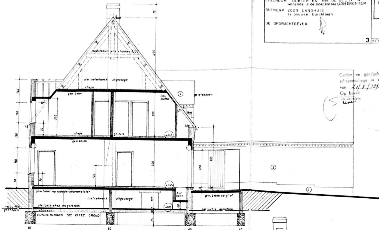
DOORSNED E-A
