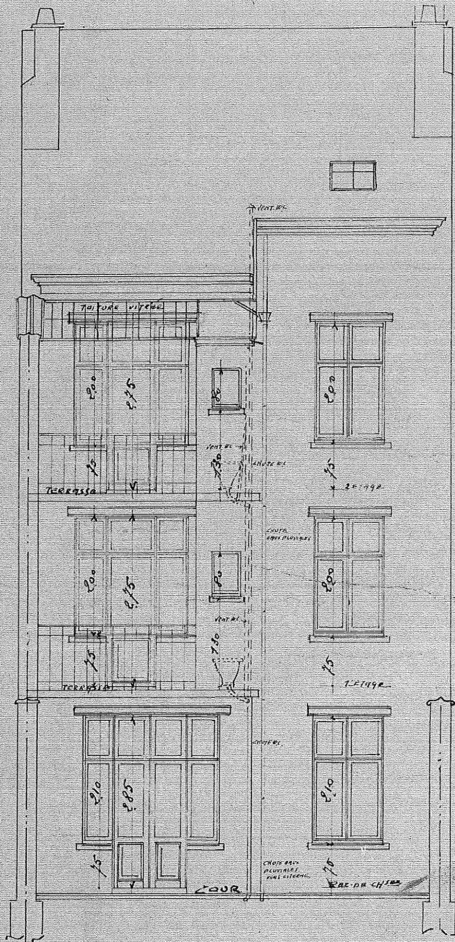
FACADE POSTERIEURE
