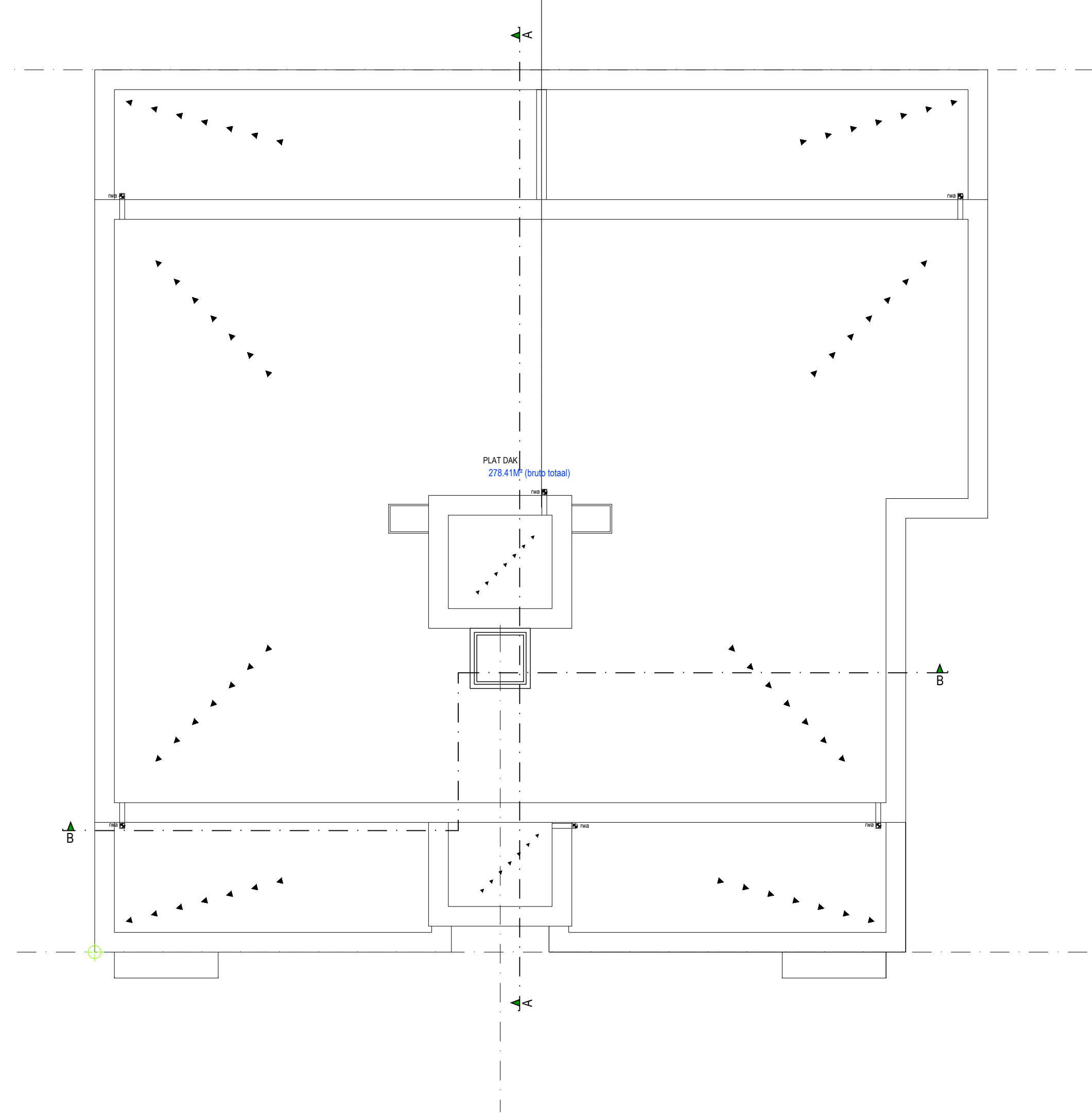
DAKPLAN - 1 / 7 5
