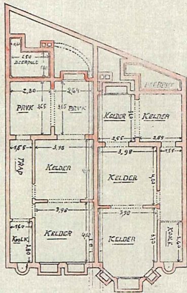
KELDERPLAN
