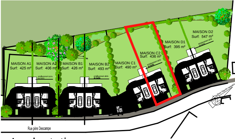
Implantation
