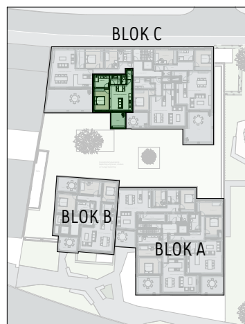
Grondplan verdieping +1
