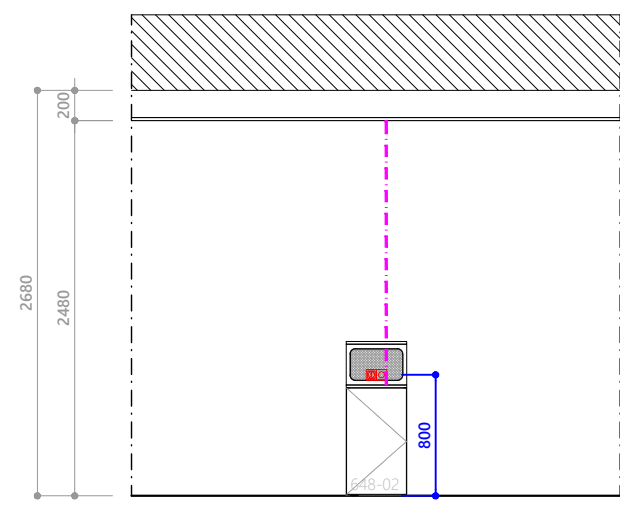
4 ELEVATION GG ELEC3 SCALE 1:50 DIMENSION IN MM
