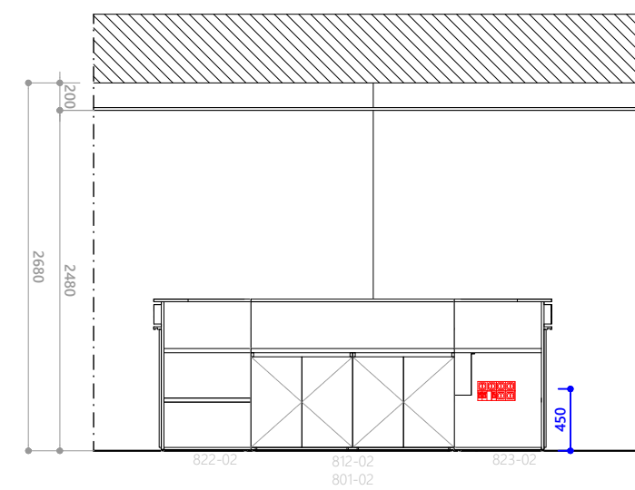
7 ELEVATION LL ELEC3 SCALE 1:50 DIMENSION IN MM
