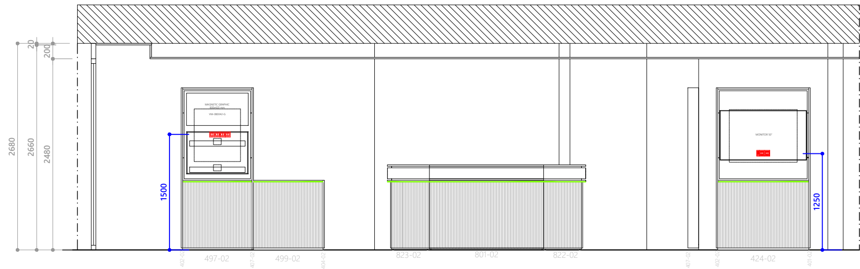
3 ELEVATION FF ELEC3 SCALE 1:50 DIMENSION IN MM
