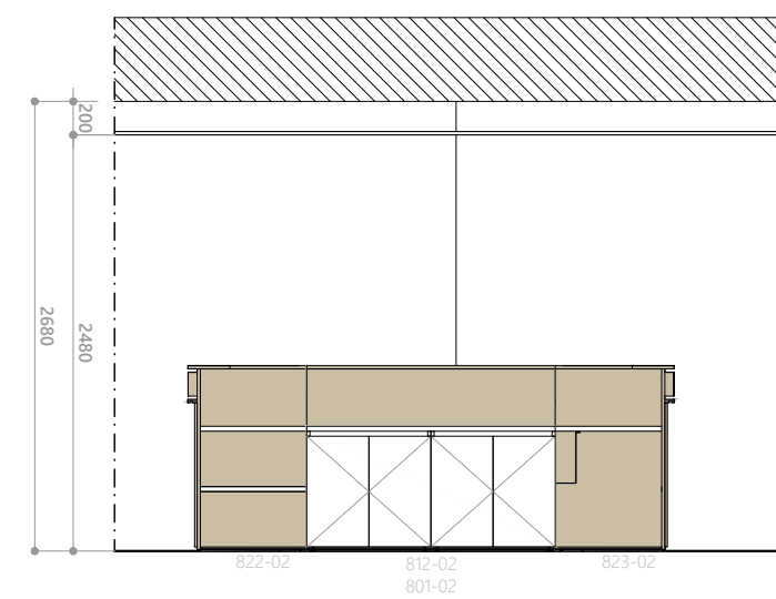
7 ELEVATION LL EL2 SCALE 1:50 DIMENSION IN MM
