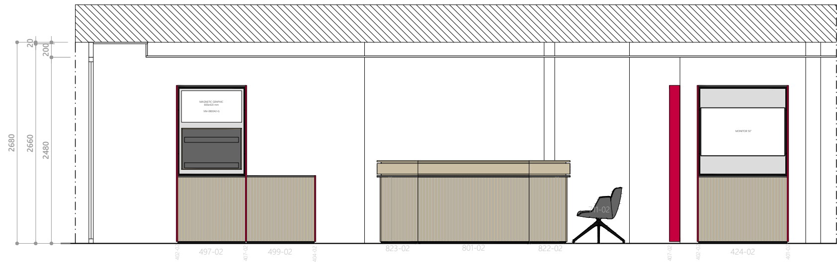
3 ELEVATION FF EL2 SCALE 1:50 DIMENSION IN MM
