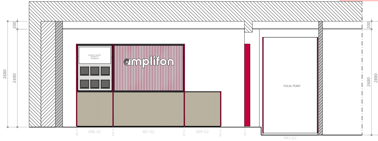
2 ELEVATION AA EL1 SCALE 1:50 DIMENSION IN MM
