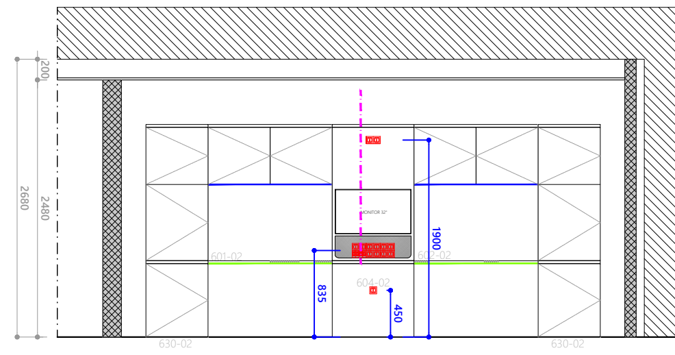
2 ELEVATION EE ELEC3 SCALE 1:50 DIMENSION IN MM
