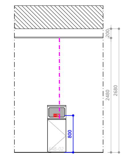
5 ELEVATION HH ELEC3 SCALE 1:50 DIMENSION IN MM
