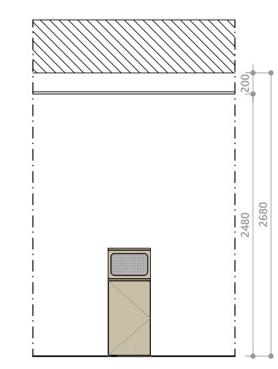
5 ELEVATION HH EL2 SCALE 1:50 DIMENSION IN MM
