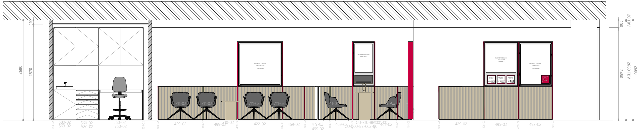
3 ELEVATION BB EL1 SCALE 1:50 DIMENSION IN MM
