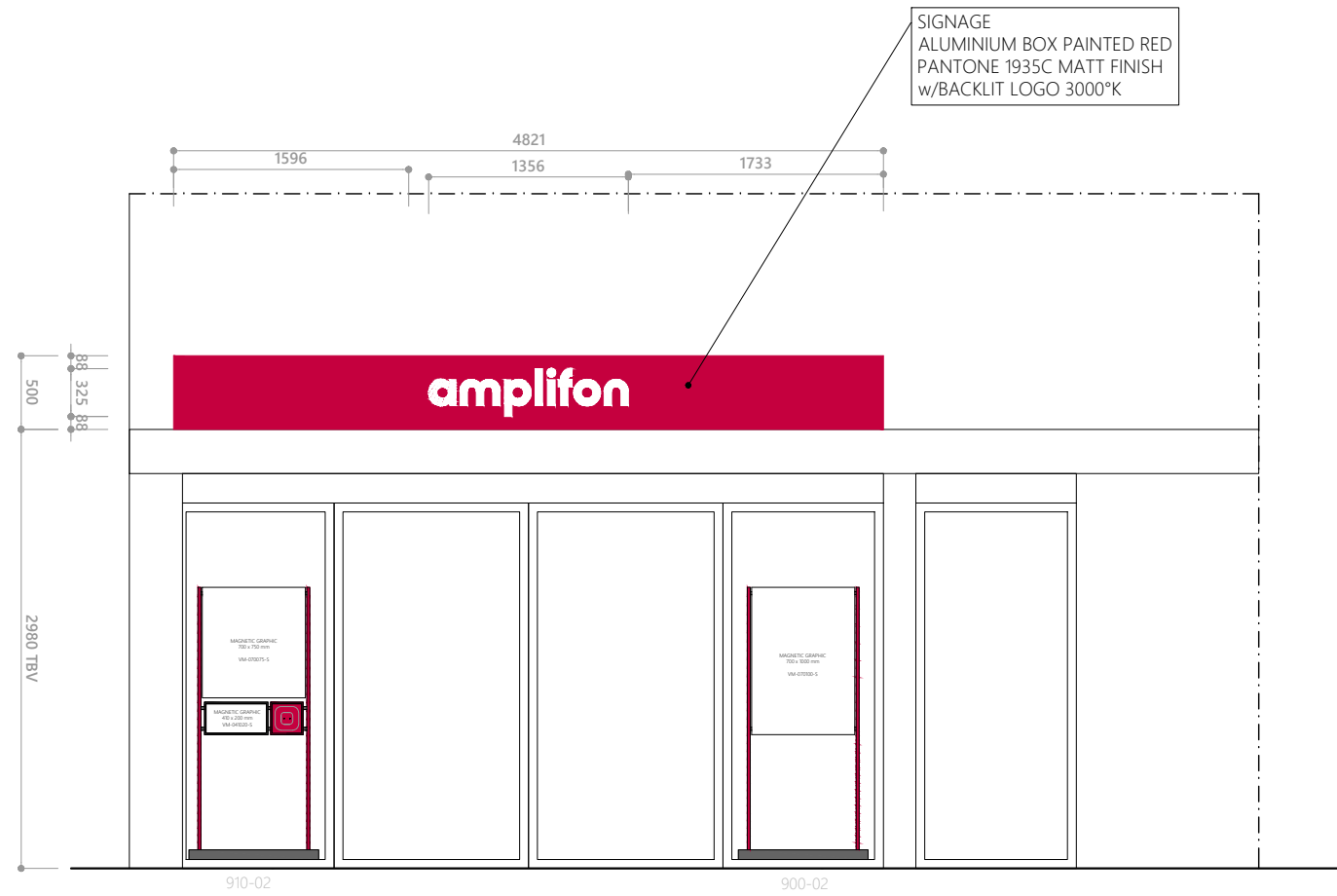
2 STOREFRONT ST1 SCALE 1:50 DIMENSION IN MM
