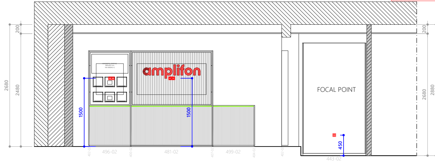
2 ELEVATION AA ELEC2 SCALE 1:50 DIMENSION IN MM
