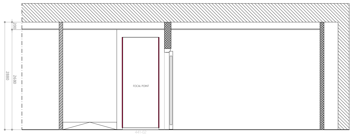
6 ELEVATION II EL2 SCALE 1:50 DIMENSION IN MM
