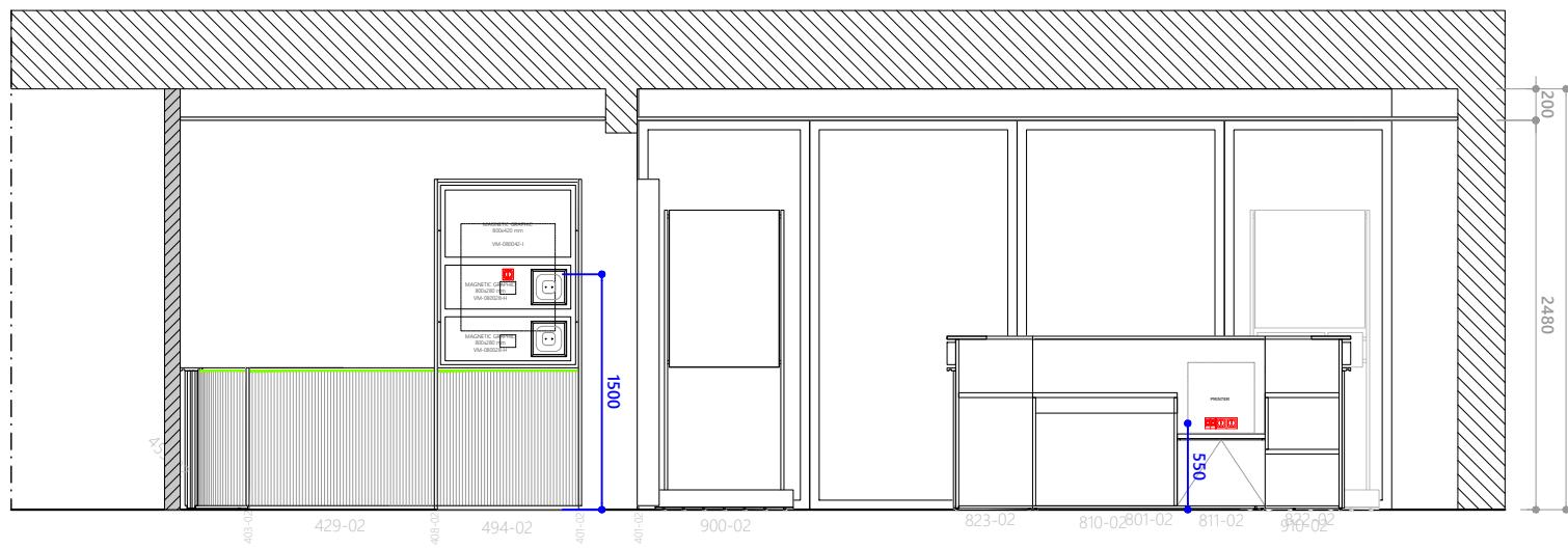
4 ELEVATION CC ELEC2 SCALE 1:50 DIMENSION IN MM
