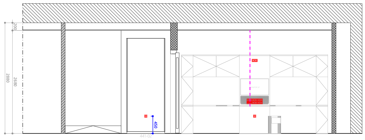
6 ELEVATION II ELEC3 SCALE 1:50 DIMENSION IN MM
