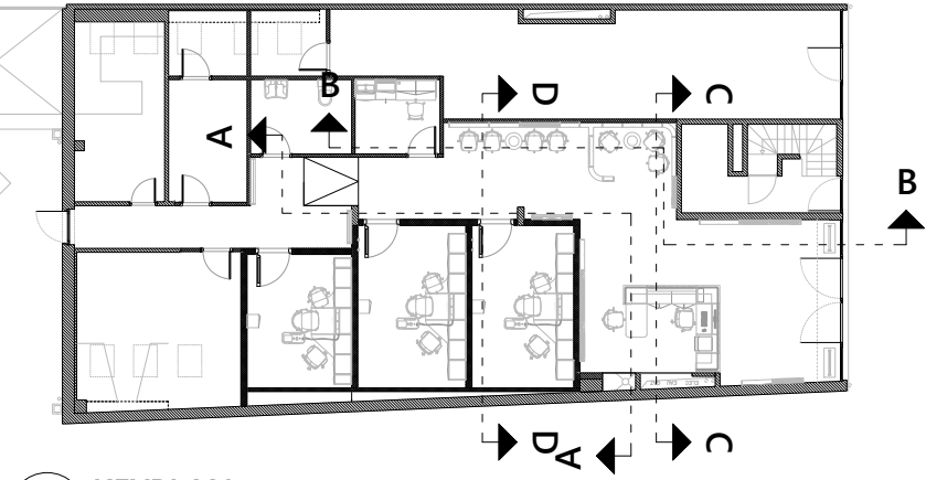
1 KEYPLAN EL1 SCALE 1:250 DIMENSION IN MM
