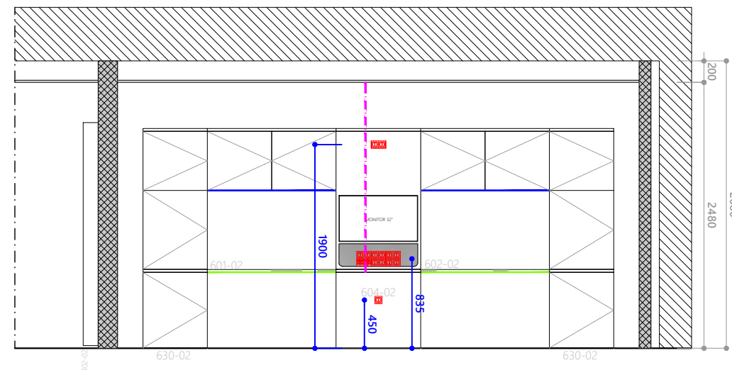
5 ELEVATION DD ELEC2 SCALE 1:50 DIMENSION IN MM
