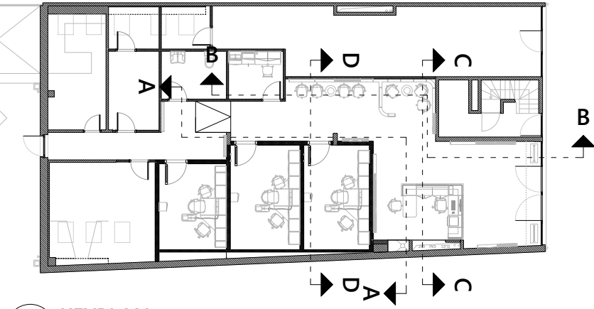
1 KEYPLAN ELEC2 SCALE 1:250 DIMENSION IN MM
