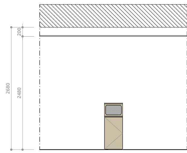
4 ELEVATION GG EL2 SCALE 1:50 DIMENSION IN MM
