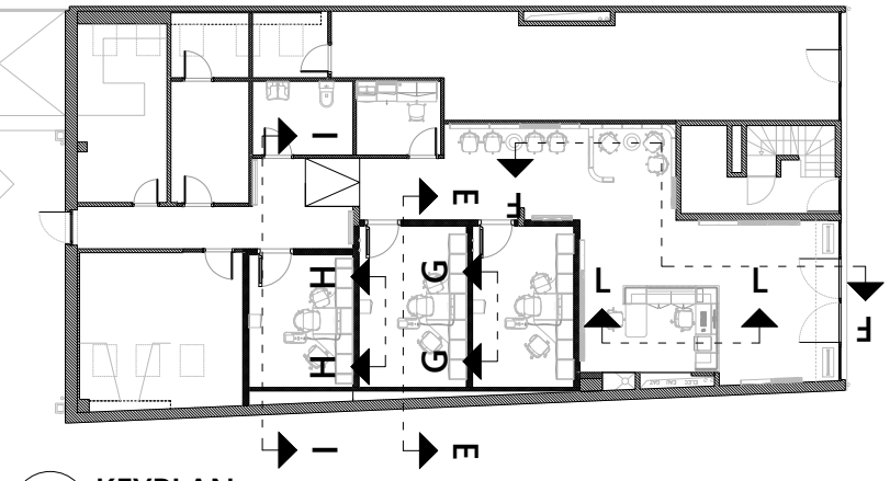
1 KEYPLAN EL2 SCALE 1:250 DIMENSION IN MM
