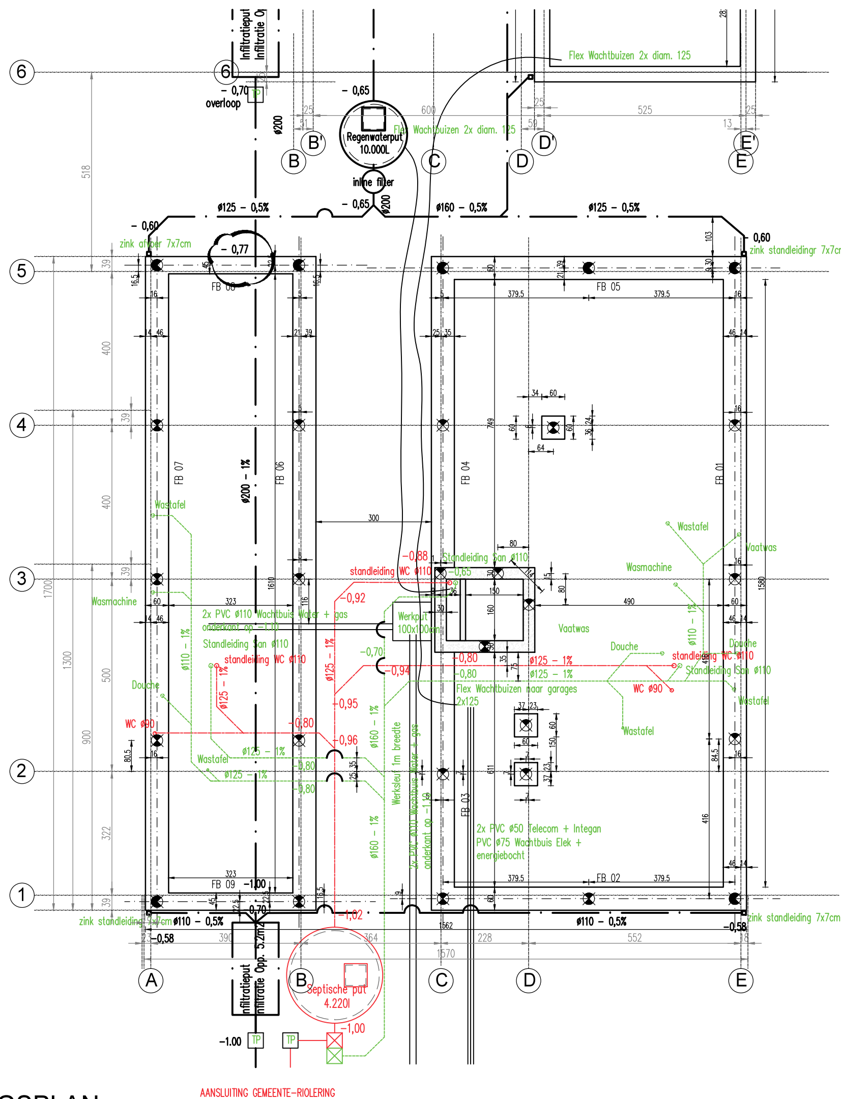
FUNDERINGSPLAN
