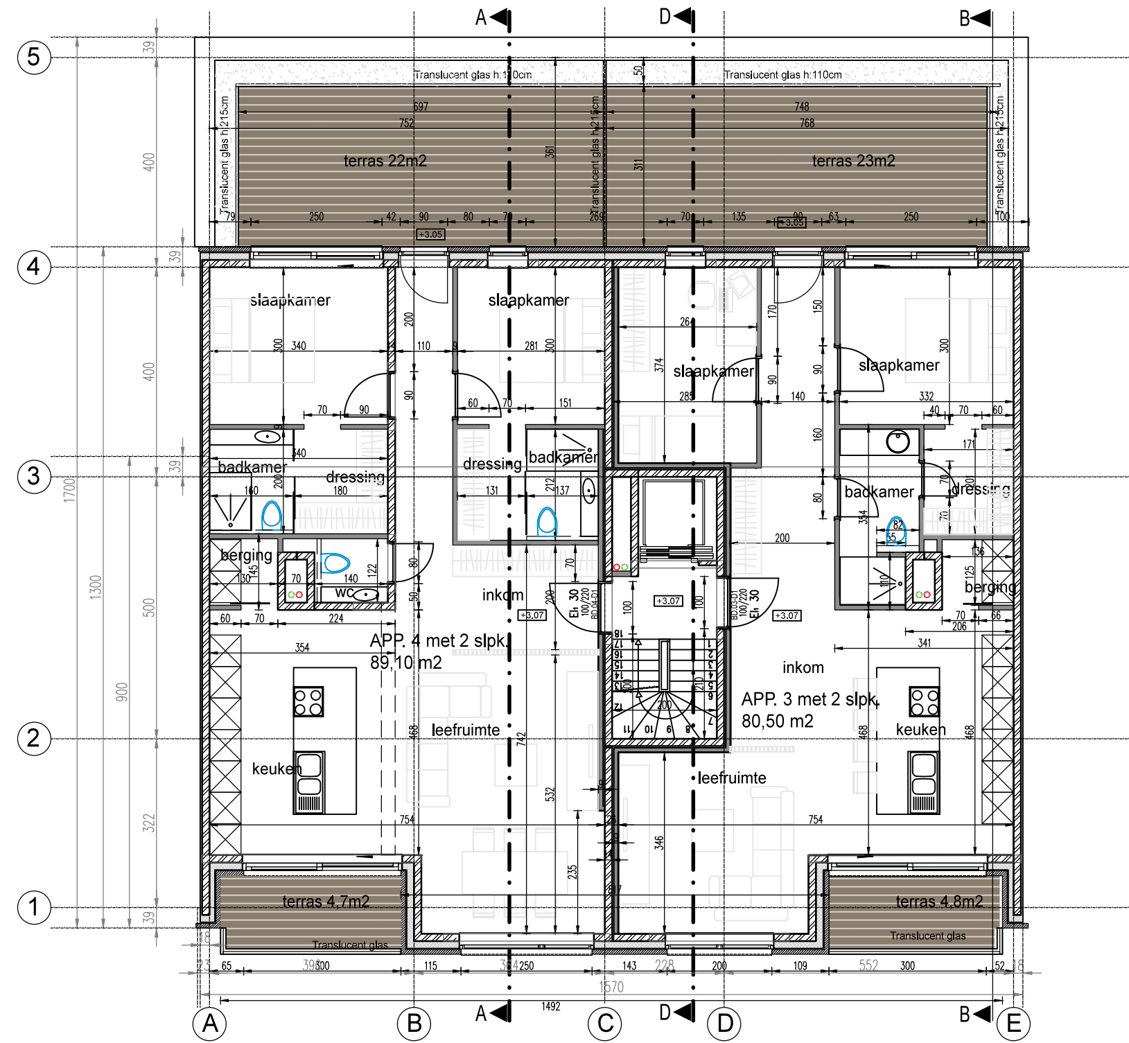
GRONPLAN 1ste VERDIEPING
