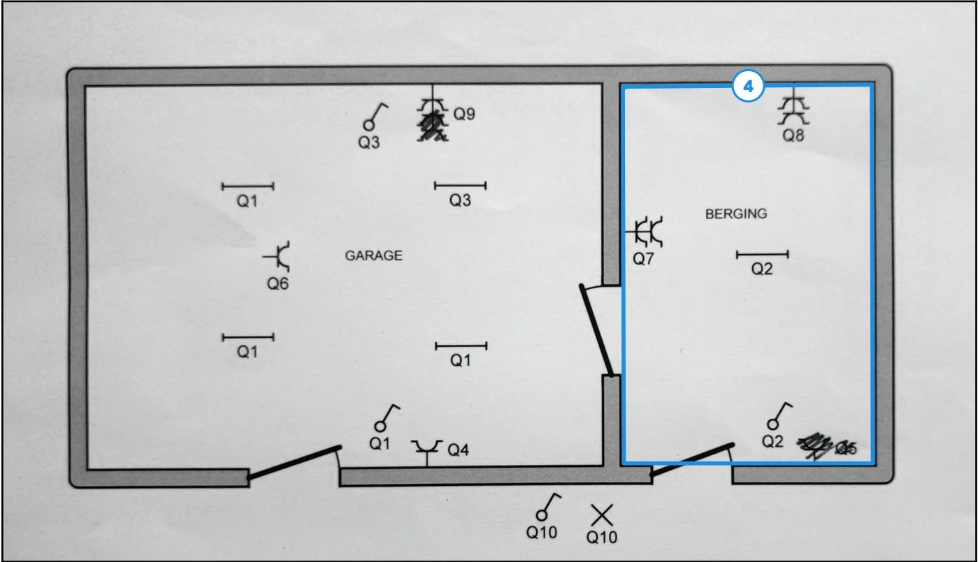
Legende van plan 1.4: Garage-berging
