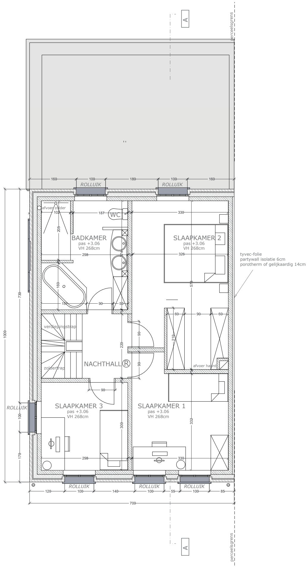
PLAN VERDIEPING
