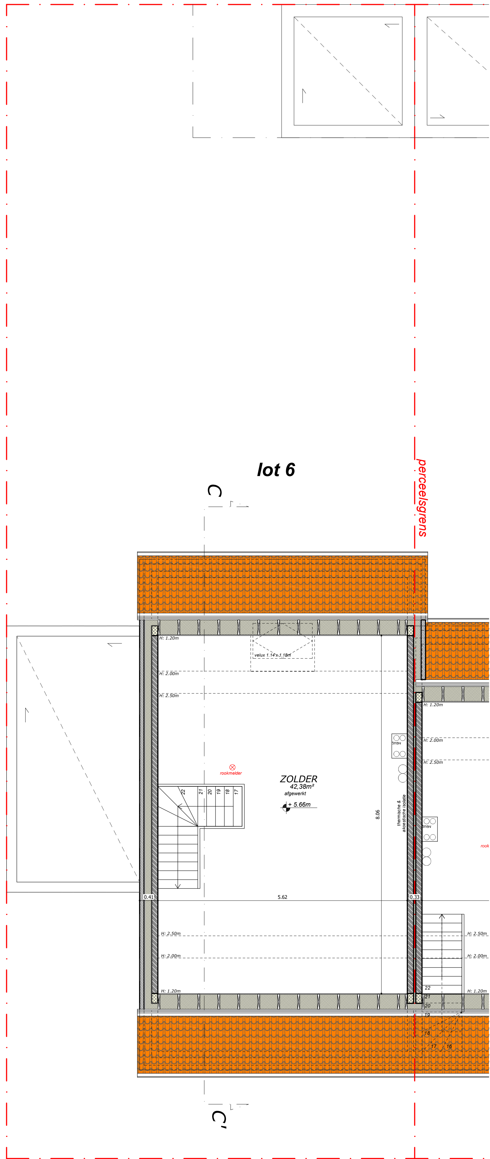
zolder verdieping
