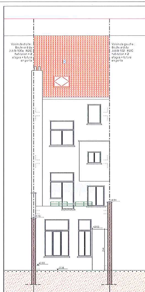
FACADE ARRIERE 1:50
