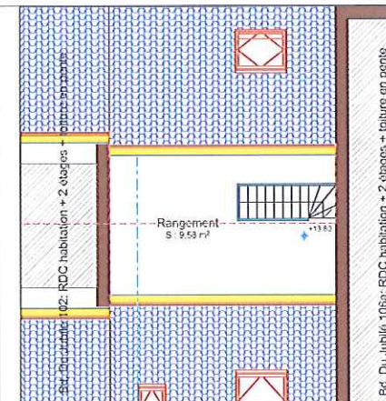
4. COMBLE 1:50
