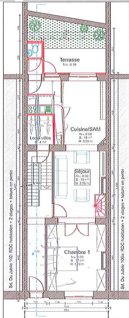
0. RE-DE-CHAUSSEE 1:50
