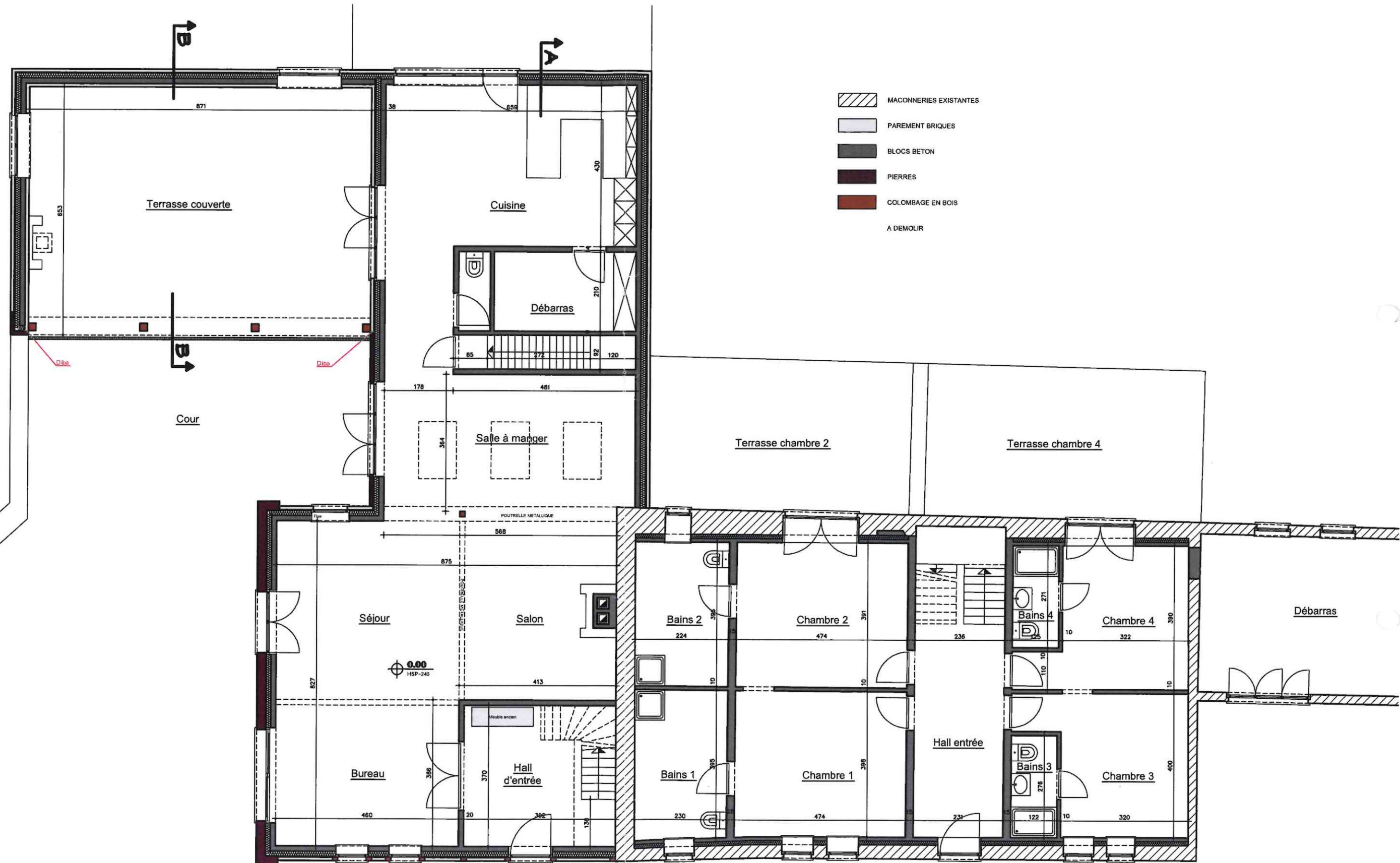
PLAN REZ
