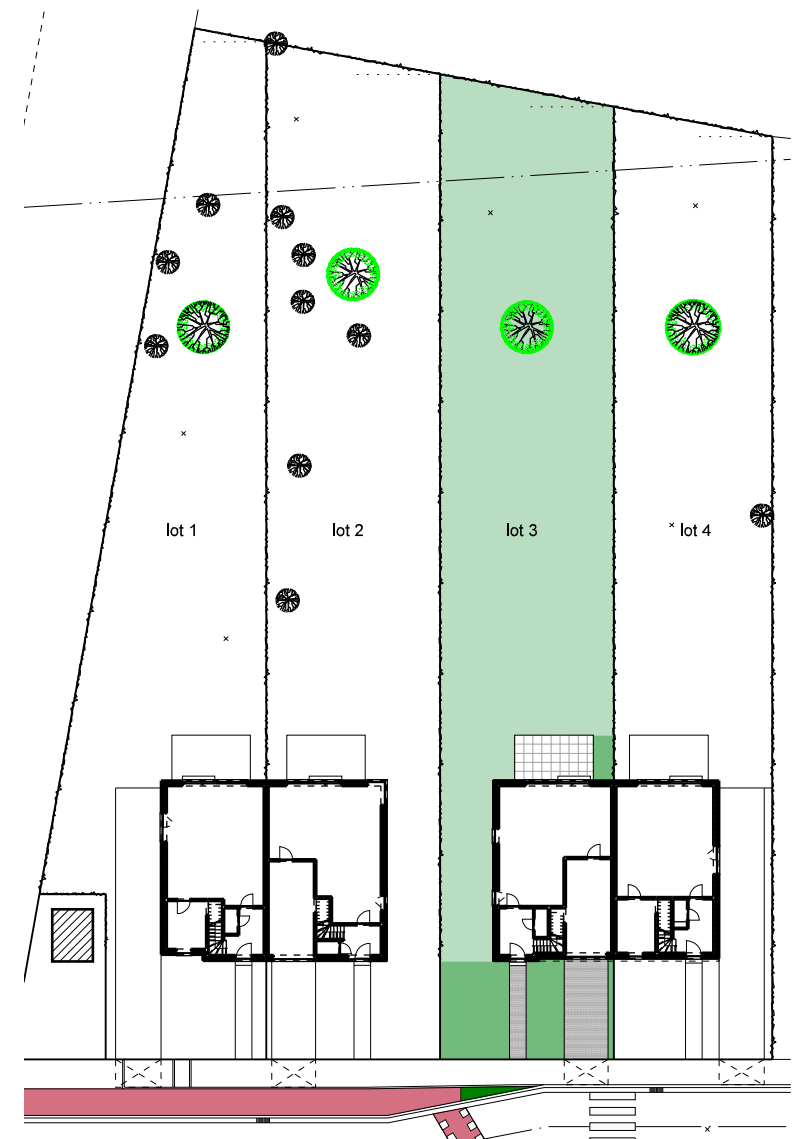
Inplanting
