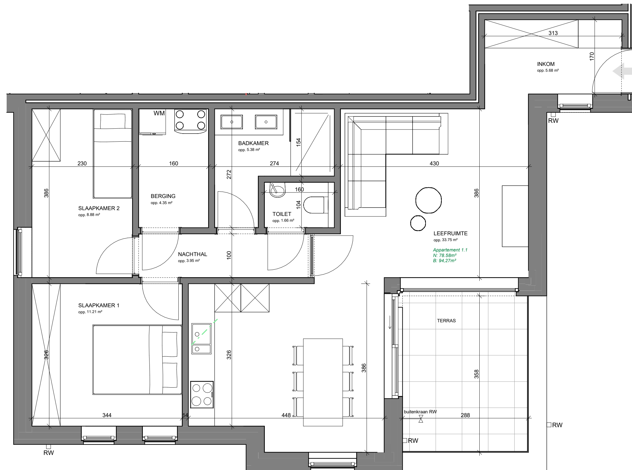
Verdieping 1 - APP 1.1
