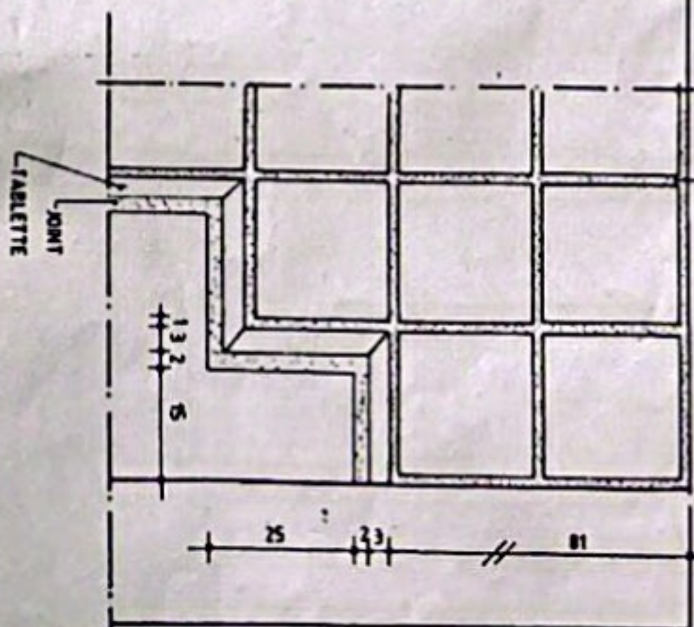
DETAIL E
