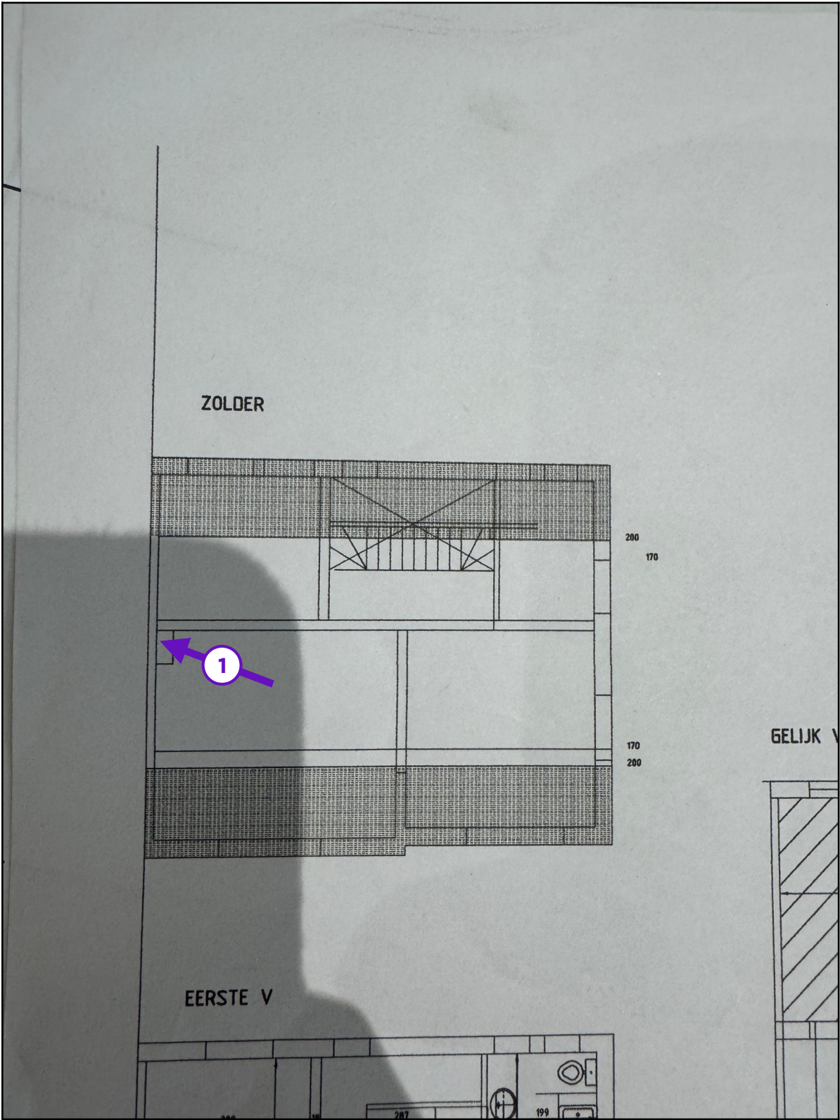
Legende van plan 2.3: Plan zolder
