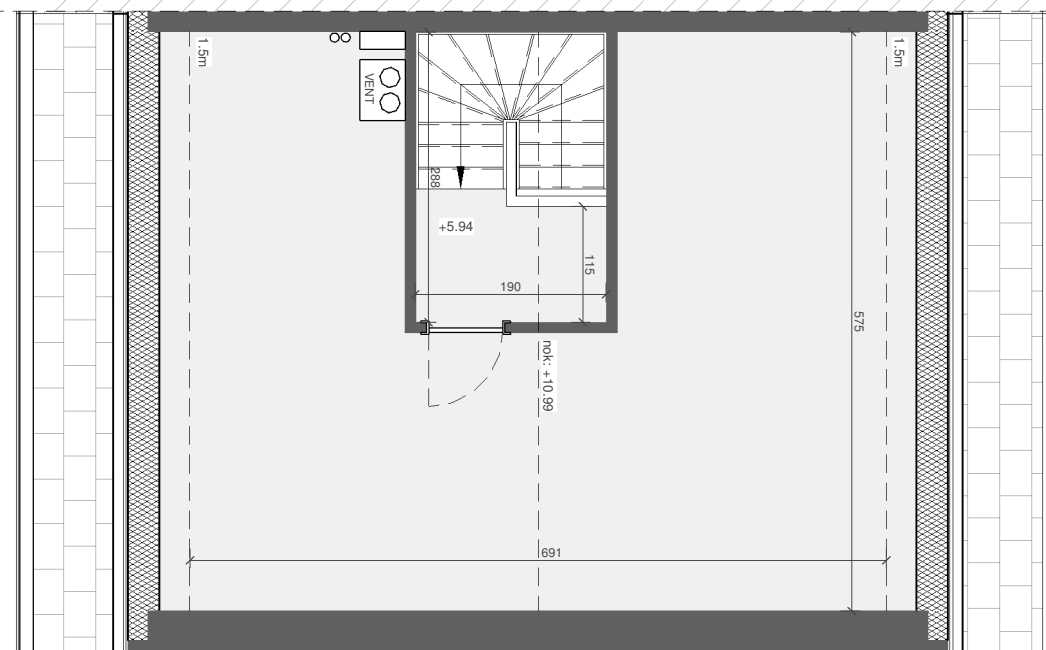
ZOLDER
