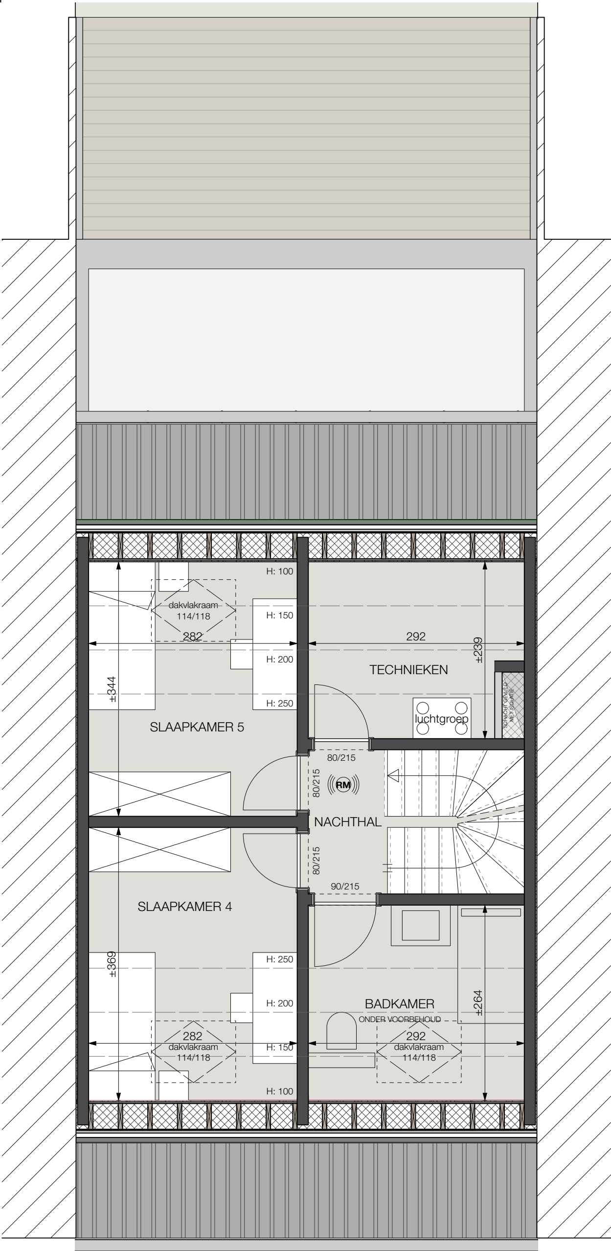
WONING 3: VERDIEPING +02
