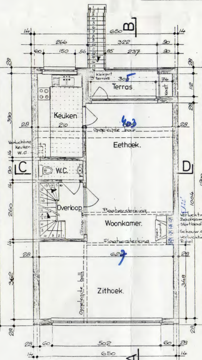
Verdieping.
