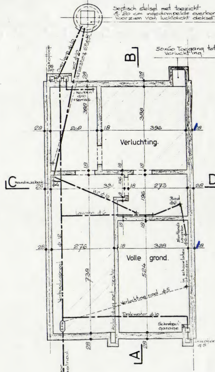
Fundering-riolering.
