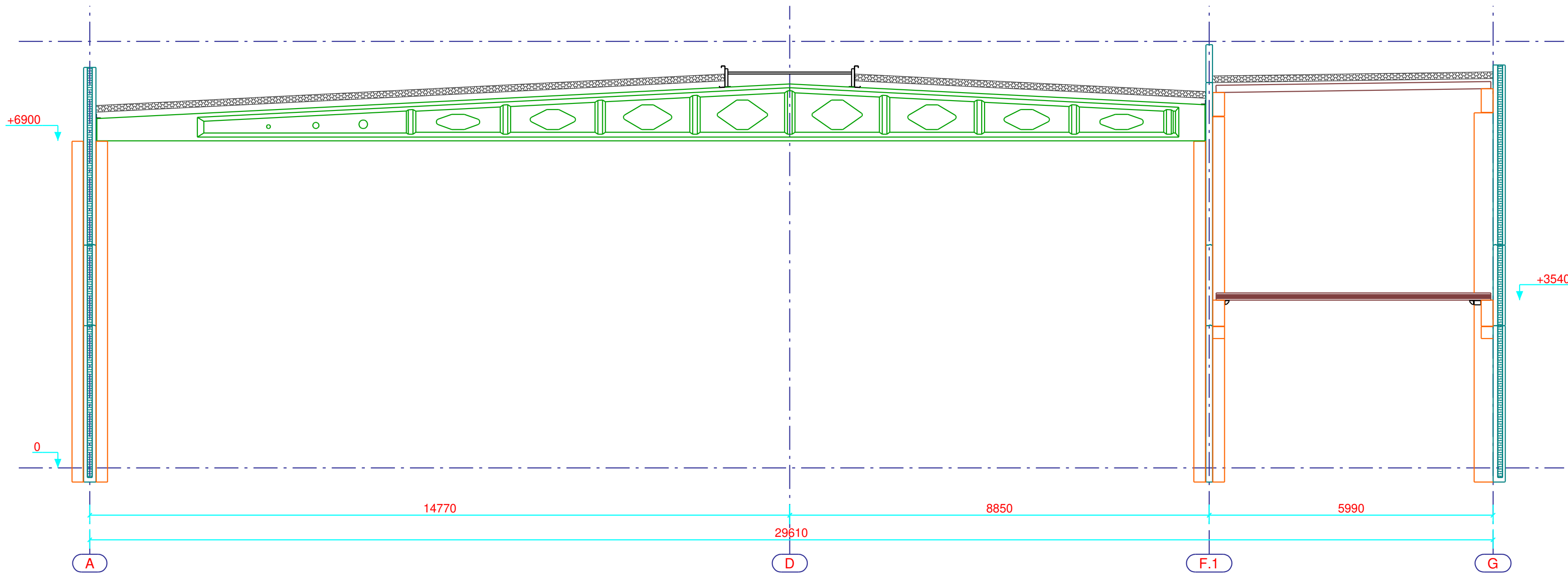
SNEDE AS 3
