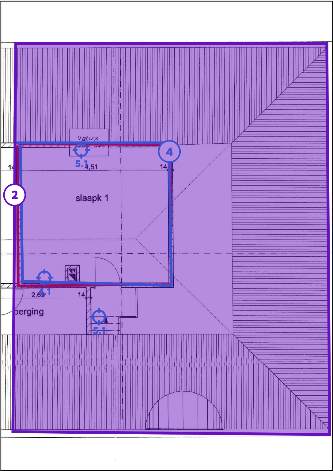
Legende van plan 1.2: AP 124 - plan zolder
