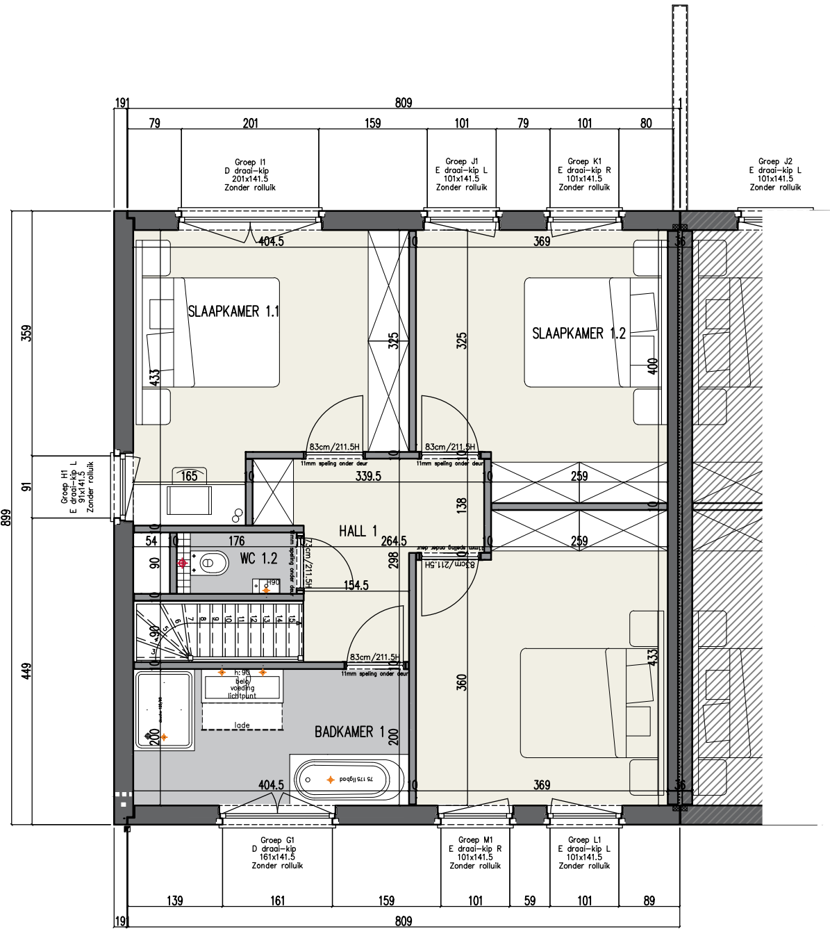
VERDIEPINGSPLAN WONING 1 Bruto opp. verd. 74,57 m²
