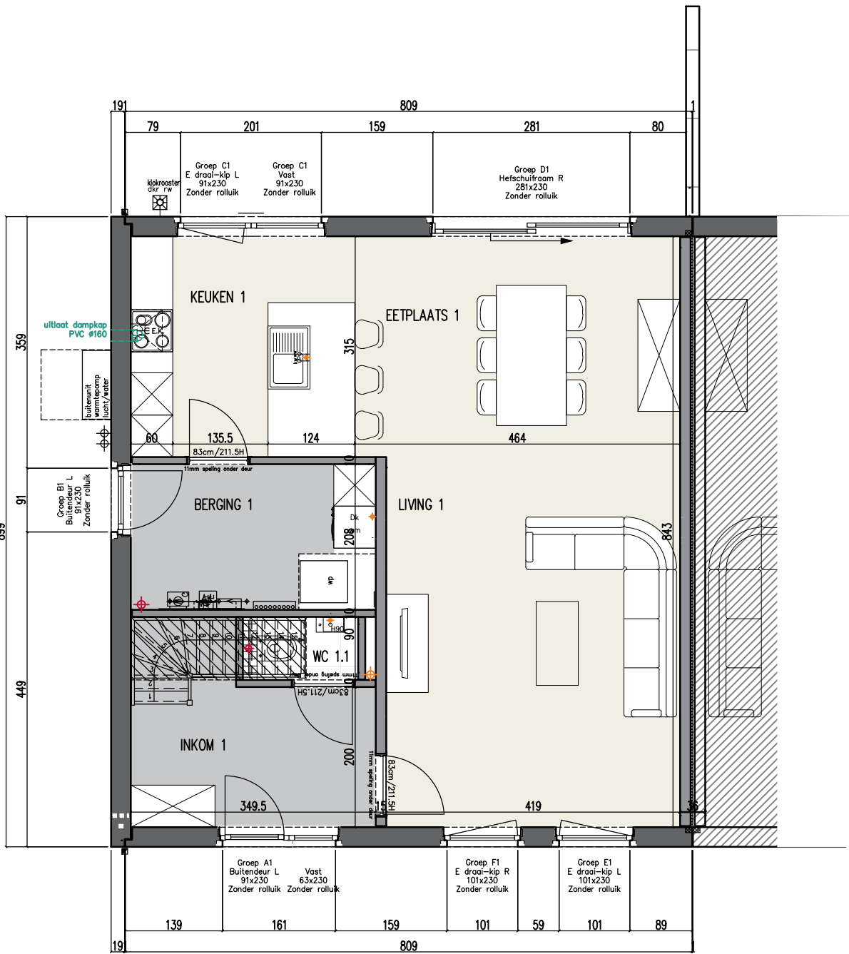
GRONDPLAN WONING 1 Bruto opp. glv. 74,57 m²
